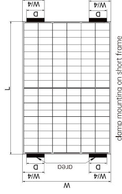
(B) CLAMP MOUNTING - SHORT FRAME
