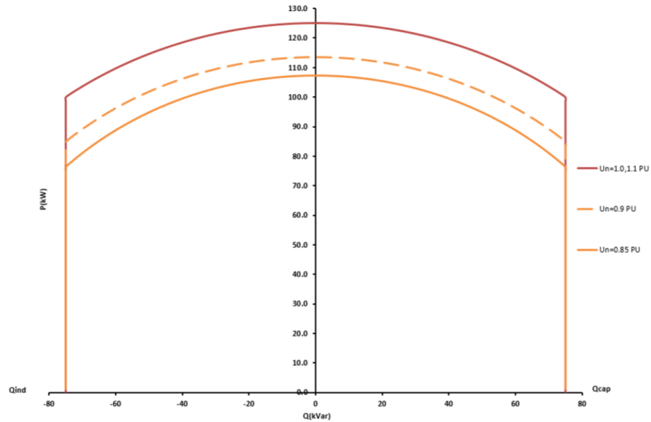
PQ Curve of SUN2000-115KTL-M2
