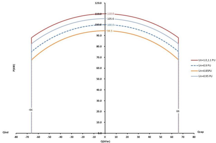
PQ Curve of SUN2000-100KTL-M2 (400Vac)
